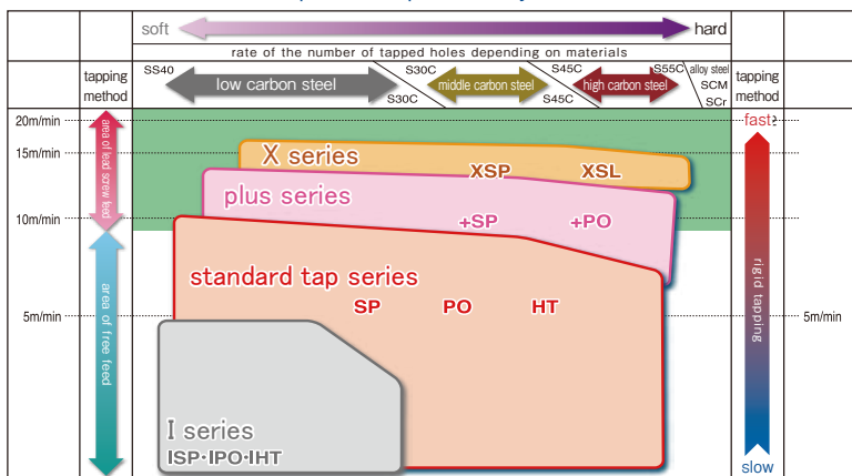
Basic concept of new products system for steels
