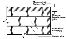
Wall Face Permissible Anchor Locations (Un-hatched Area)
