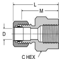
FEMALE CONNECTOR 66C Reference SAE 060103 BA
