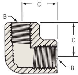
90° FEMALE PIPE ELBOW- Extruded NPTF - Dryseal Ref. SAE 130238
