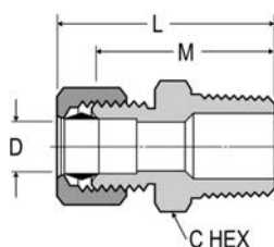
MALE CONNECTOR 68C Reference SAE 060102 BA
