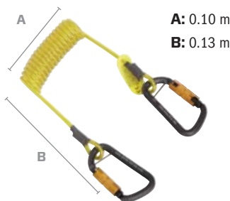
HOOK2HOOK COIL TETHER - 1500063
