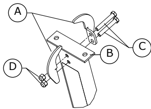
Figure 11 - Pass-Through Brackets
